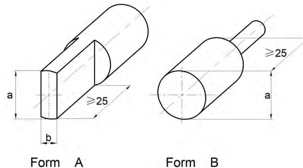
A型和B型模拟量规
