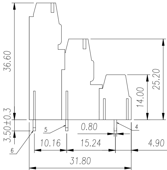
General Tolerances
