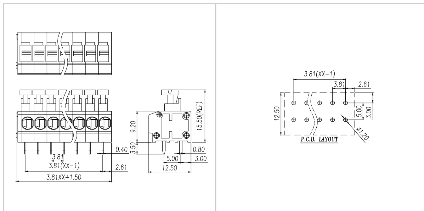
PCB opening diagram
